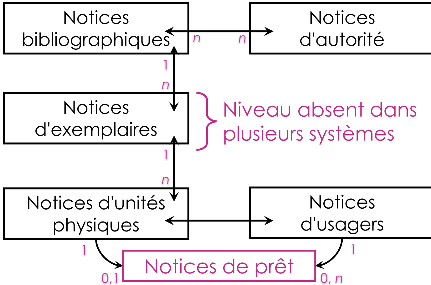
Figure 3-1. Design of Library Information System Files (Kochtanek et Matthews, 2002, p. 30)
